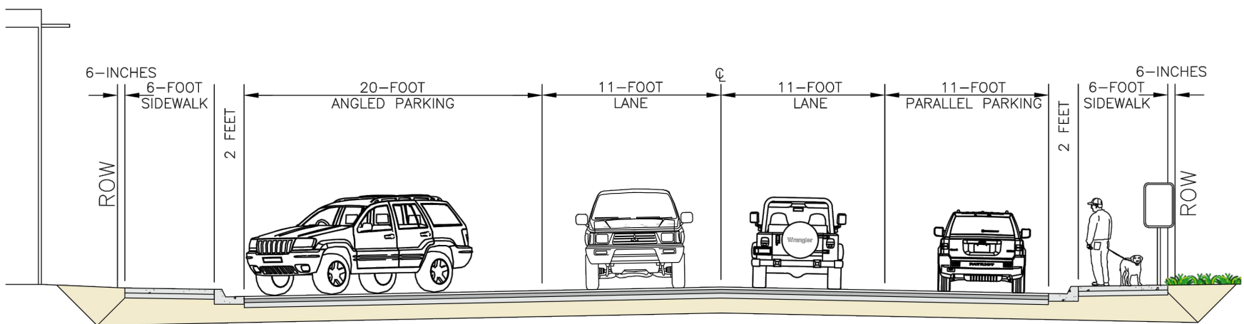
TYPICAL SECTION, BLOCK 2
