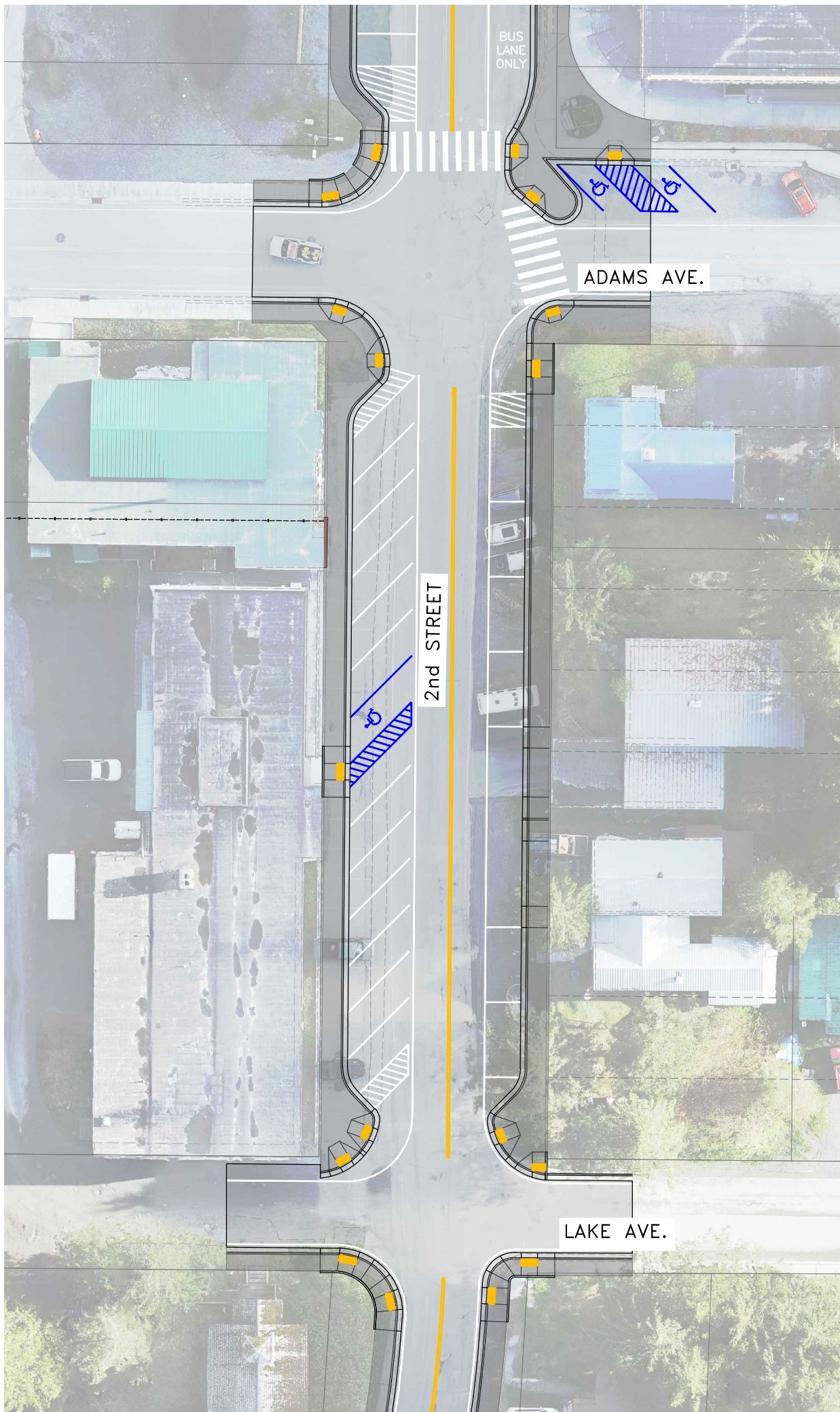
PLAN VIEW
